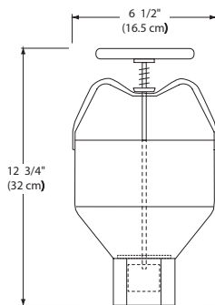
Type K Donut Depositor
