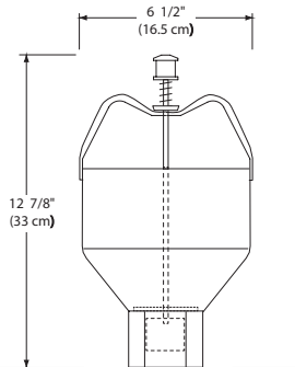
Type K Pancake Dispenser
